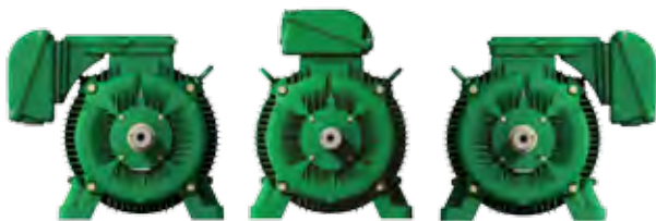
Figure 24 - Terminal box mounted on both sides and on top (frames 225 to 355)
