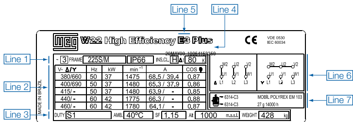
Figure 14 - Nameplate for multi-voltage design
