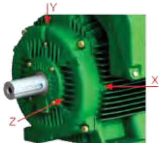
Figure 6 - Flat surfaces for vibration checking on the DE side (frames 225 to 355)
