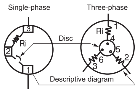
Figure 7.7 - Internal view of the thermal protector
