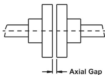
Figure 1c - Axial alignment (concentricity).
