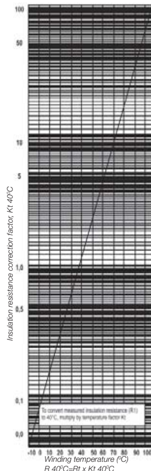
Graphic 1. Variation of insulation resistance with the temperature.
